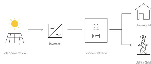
PV + sonnenBatterie eco (with an additional PV inverter)
